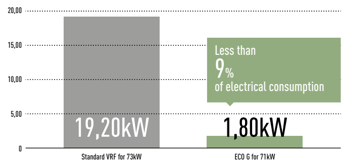
Limited electricity area. Comparison of electrical consumption on a 71kW outdoor unit.
