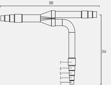
Discharge tubing
