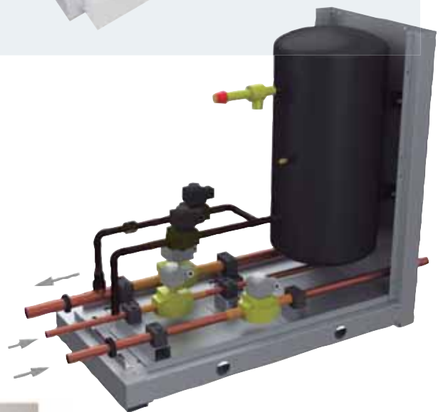
Leak detectors
