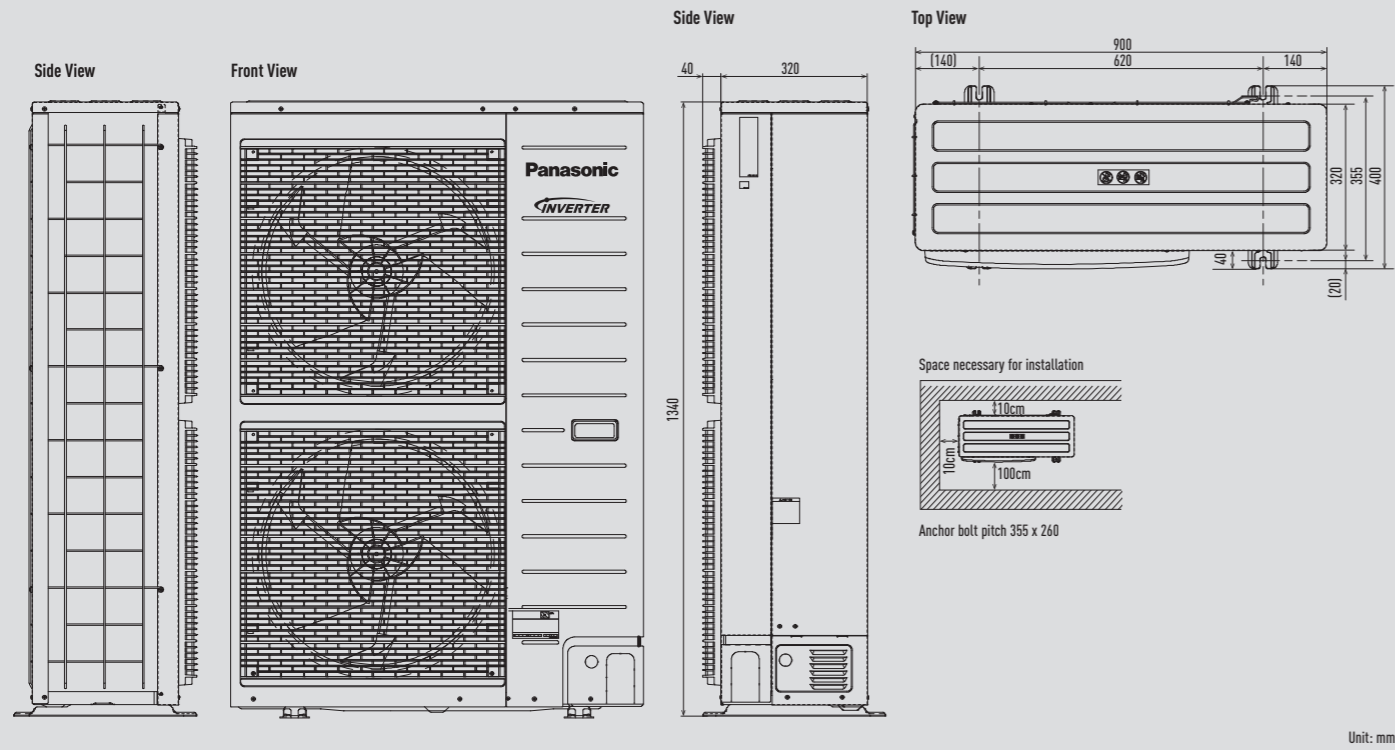
Bi-bloc outdoor unit from 9 to 16kW
