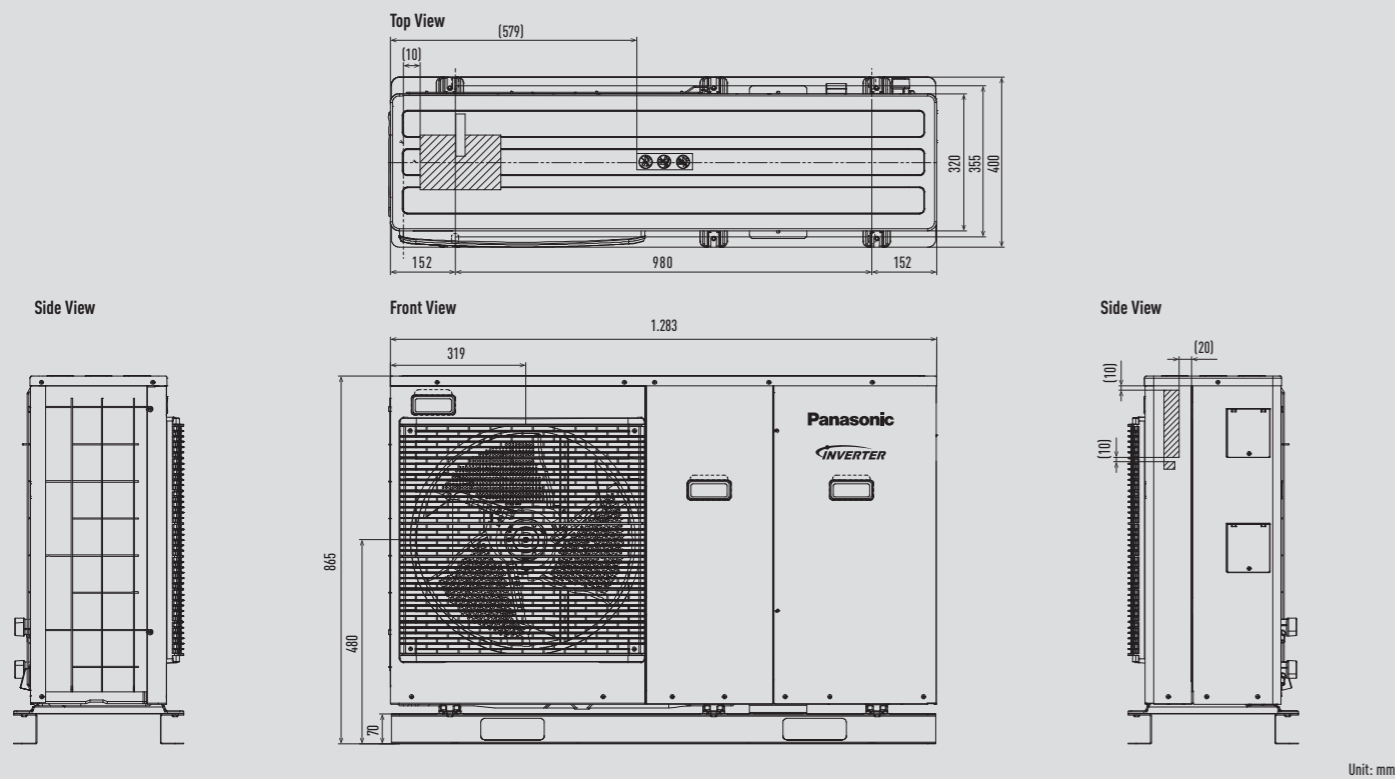
Mono-bloc outdoor unit from 5 to 9kW
