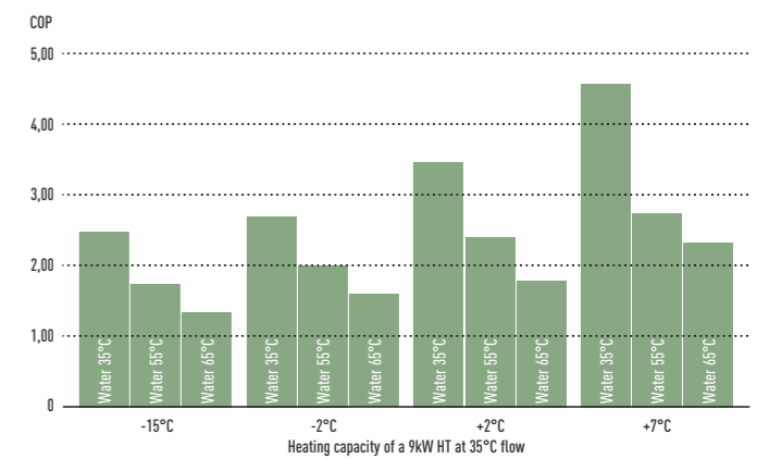
COP (Coefficient of Performance) of a 9kW HT (WH-MHF09G3E5).
