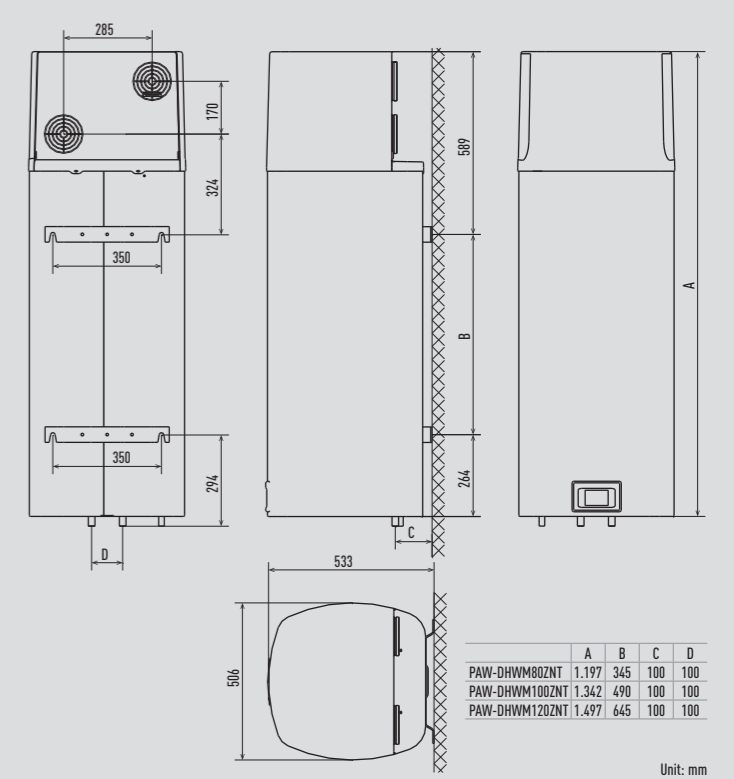
Aquarea DHW Wall mounted
