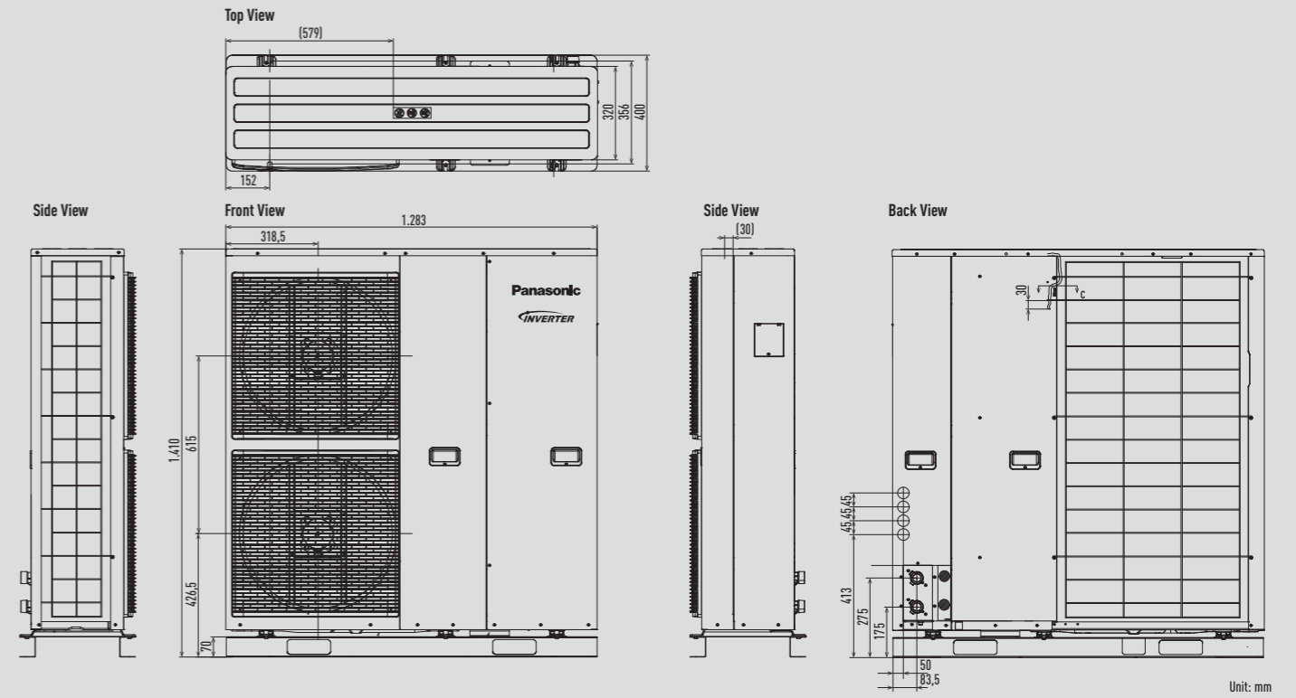
Bi-bloc Super Quiet outdoor unit and Mono-bloc outdoor unit from 9 to 16kW
