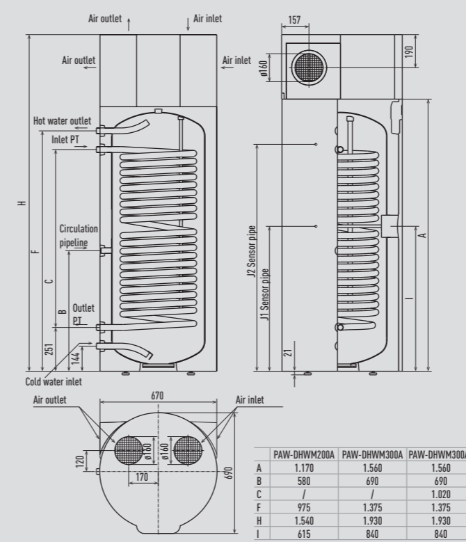
Aquarea DHW Floor standing
