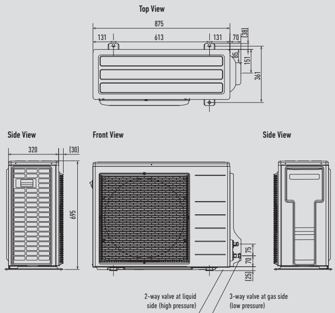
CU-E15PKEA / CU-E18PKEA
