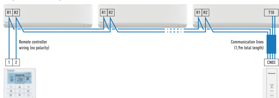
Example when there are multiple indoor units.
