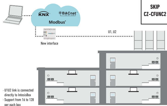
NEW Interface with P-communication bus
