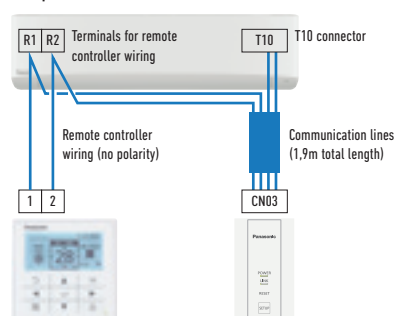
Example when there is 1 indoor unit.
