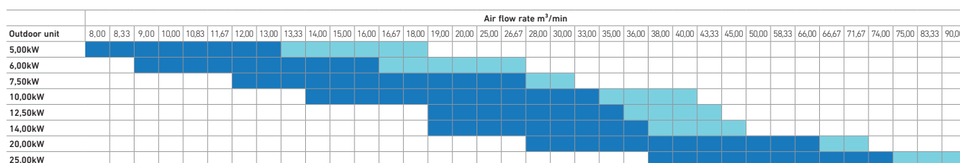
Standard range of air flow rate under standard conditions (air intake temperature in cooling mode from 18 to 32°C DB).
