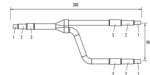
Liquid tubing
