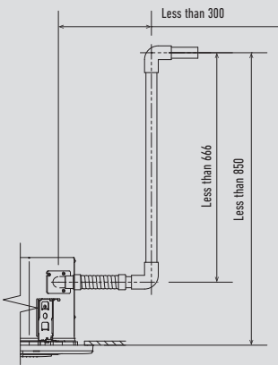
Raise dimension of drain tube
