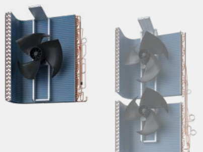
Conventional model with two fans.
