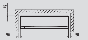
Minimum space requirements for installation
