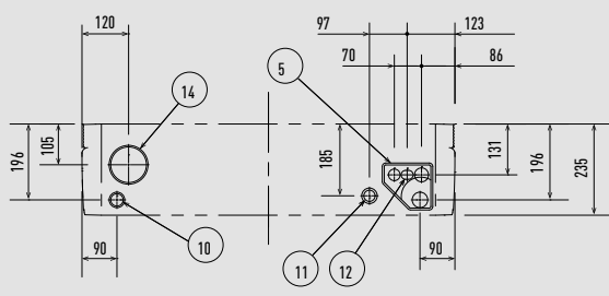
Tubing hole position on wall surface (figure shows view from front)
