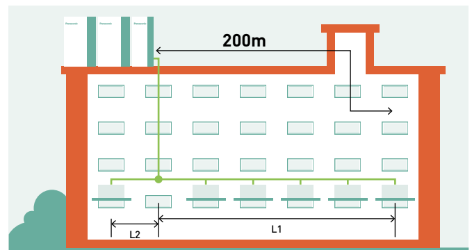
L1 = Longest pipe run. L2 = Shortest pipe run. L1 - L2 = Maximum 50 m.
