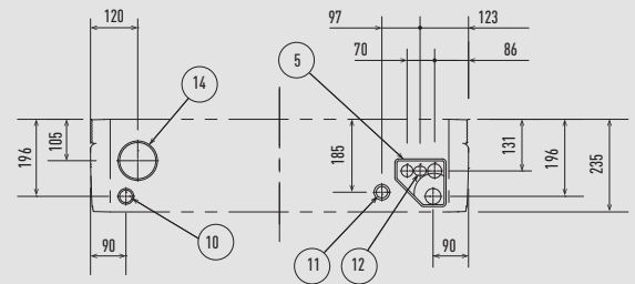
Tubing hole position on wall surface (figure shows view from front)
