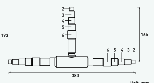
Liquid piping
