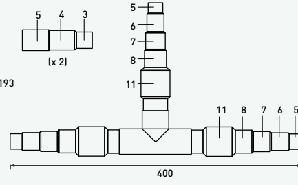
Discharge piping
