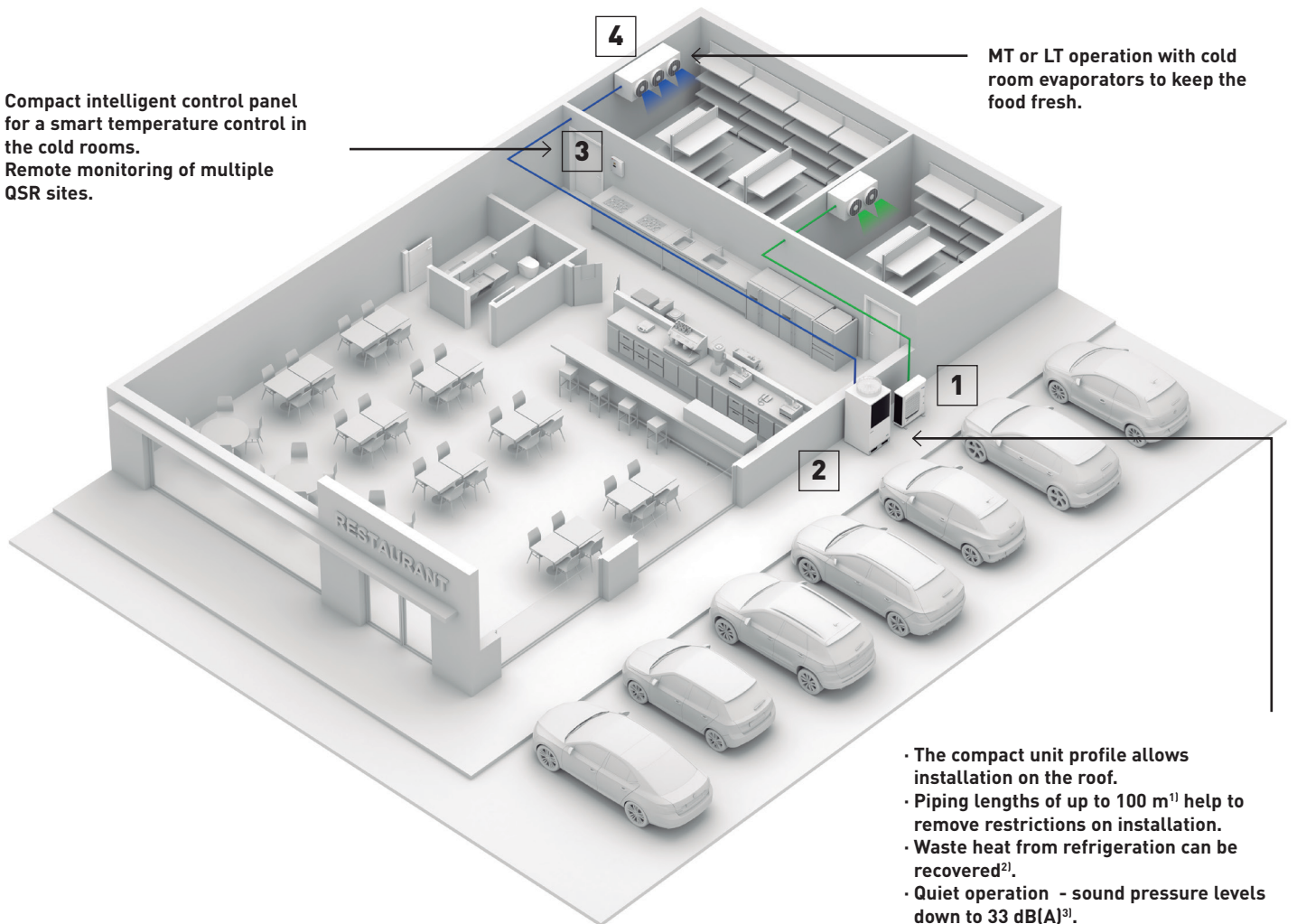
1 2 HP MT/LT condensing unit (OCU-CR200VF5A).
