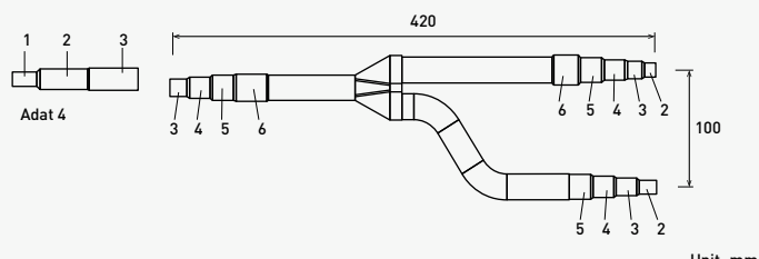
Liquid piping
