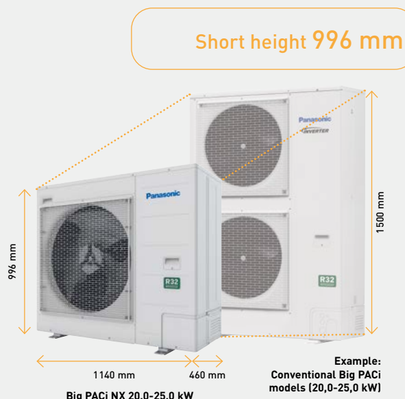
Big PACi NX 20,0-25,0 kW
