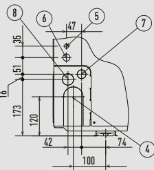
View Z
