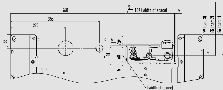
View E
