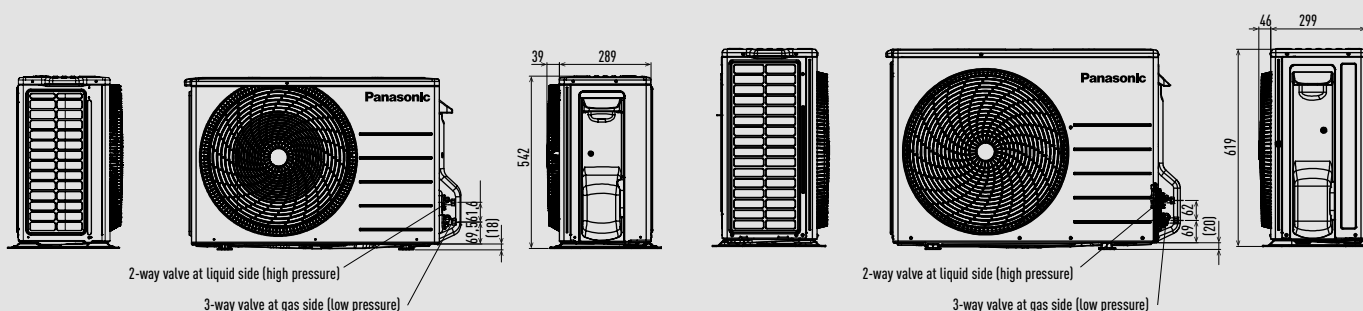
Side view
