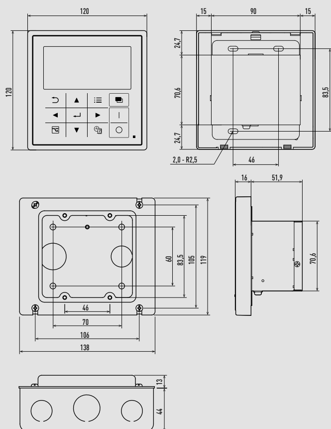
CZ-64ESMC3 system controller with weekly timer.
