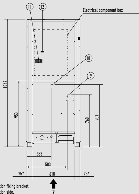
View E
