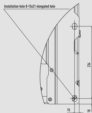
View D
