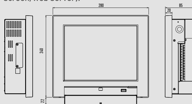
CZ-256ESMC3 intelligent controller (touch screen/web server).
