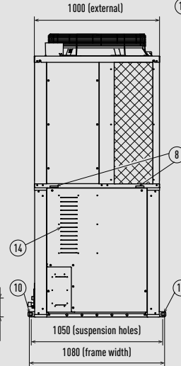
Left view
